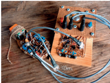
Atari Punk Flasher.
